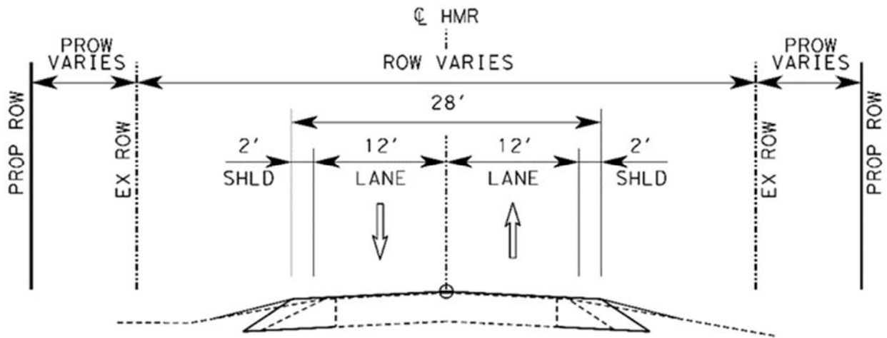
Proposed typical section along Hairy Man Rd.
