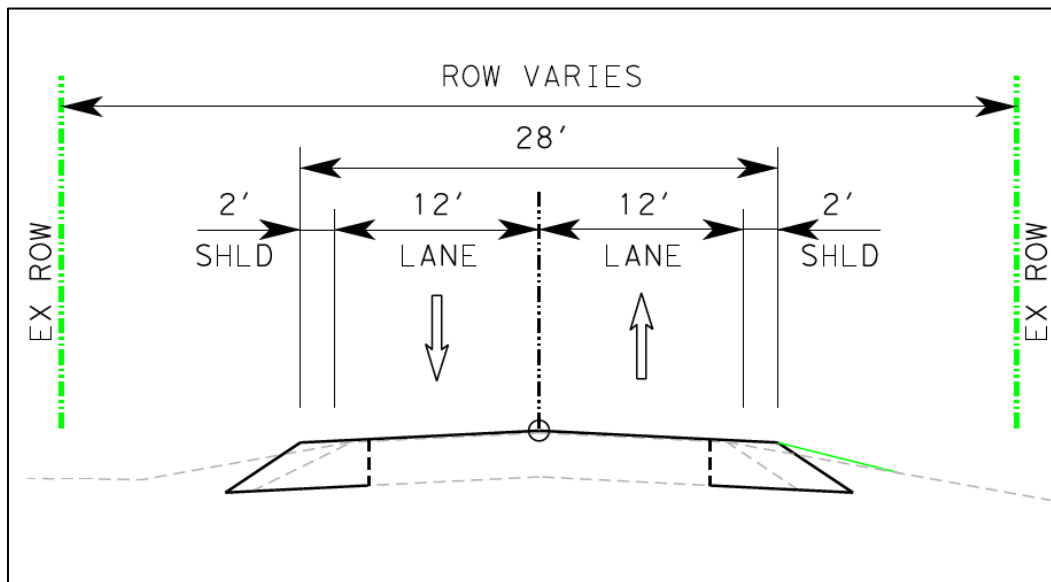
Proposed typical section along Hairy Man Rd.
